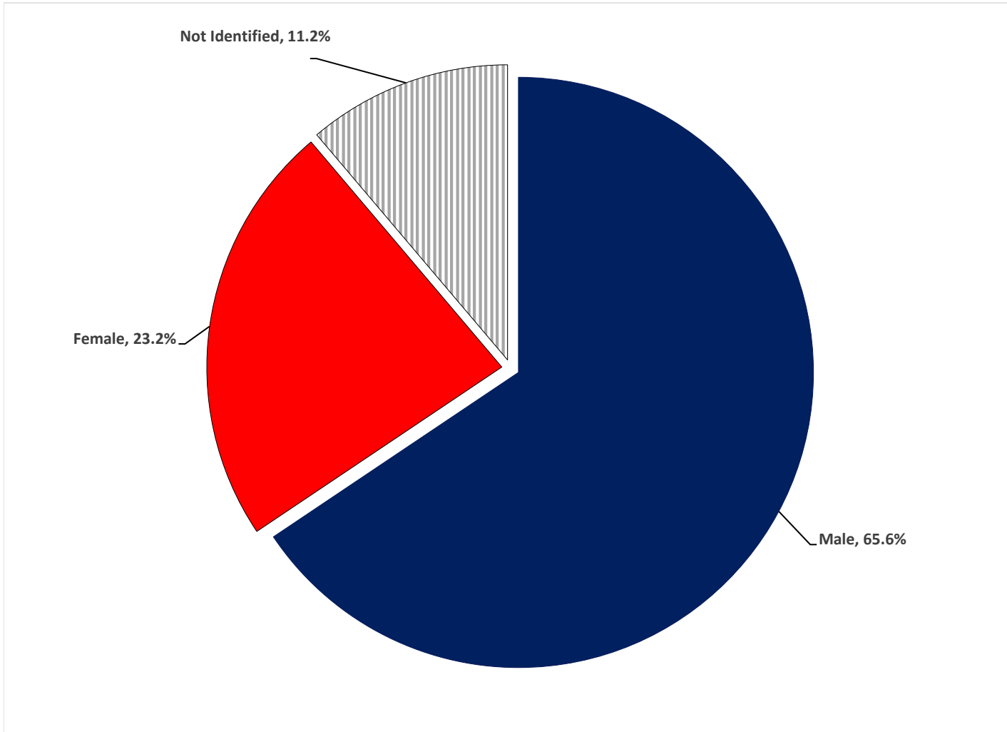
CHART 6 - GENDER OF OFFENDERS 2018
